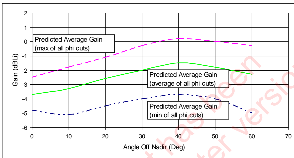
Figure 5.9: Sarsat-METOP 406 MHz SARR and SARP Receive Antenna (CRA) Gain Pattern (at receiver input)
