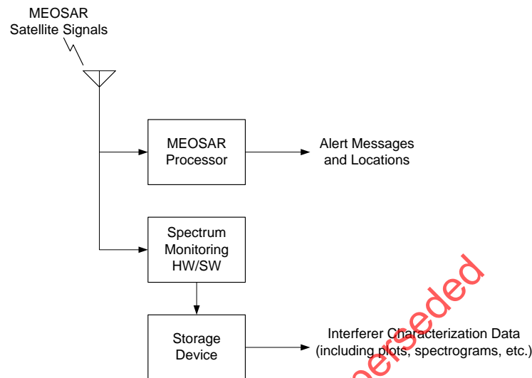
Figure 4.1: Test Apparatus for Interference Evaluation
