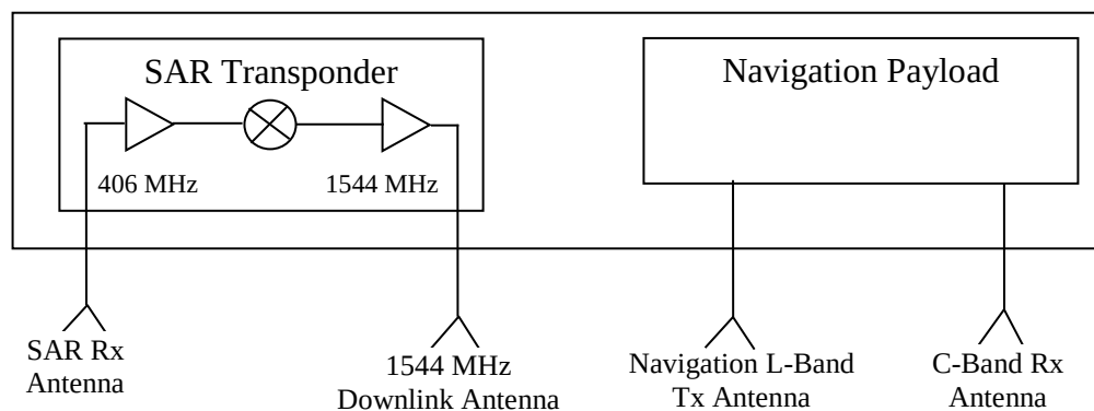
Figure 2.3: SAR/Galileo Payload Functions
