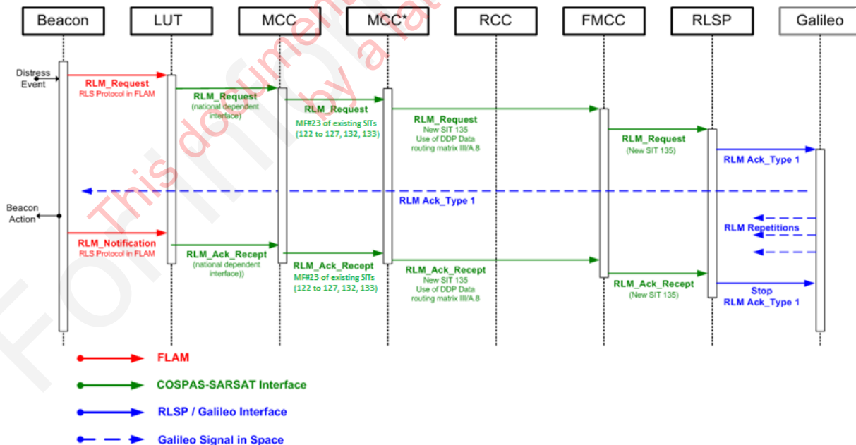
Figure 7.6: RLS Data Exchange Overview
