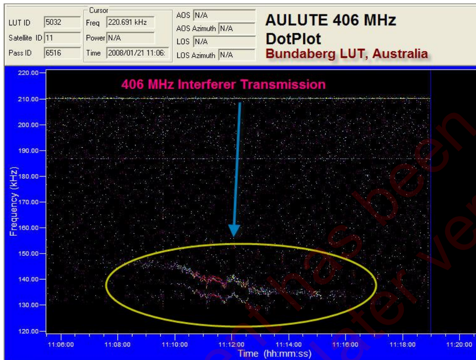
Figure 1.7: 406 MHz Interferer Location Information
