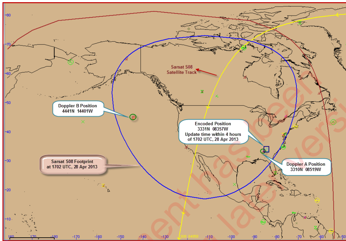
Figure 6.7: LEOSAR Position Conflict Alert
