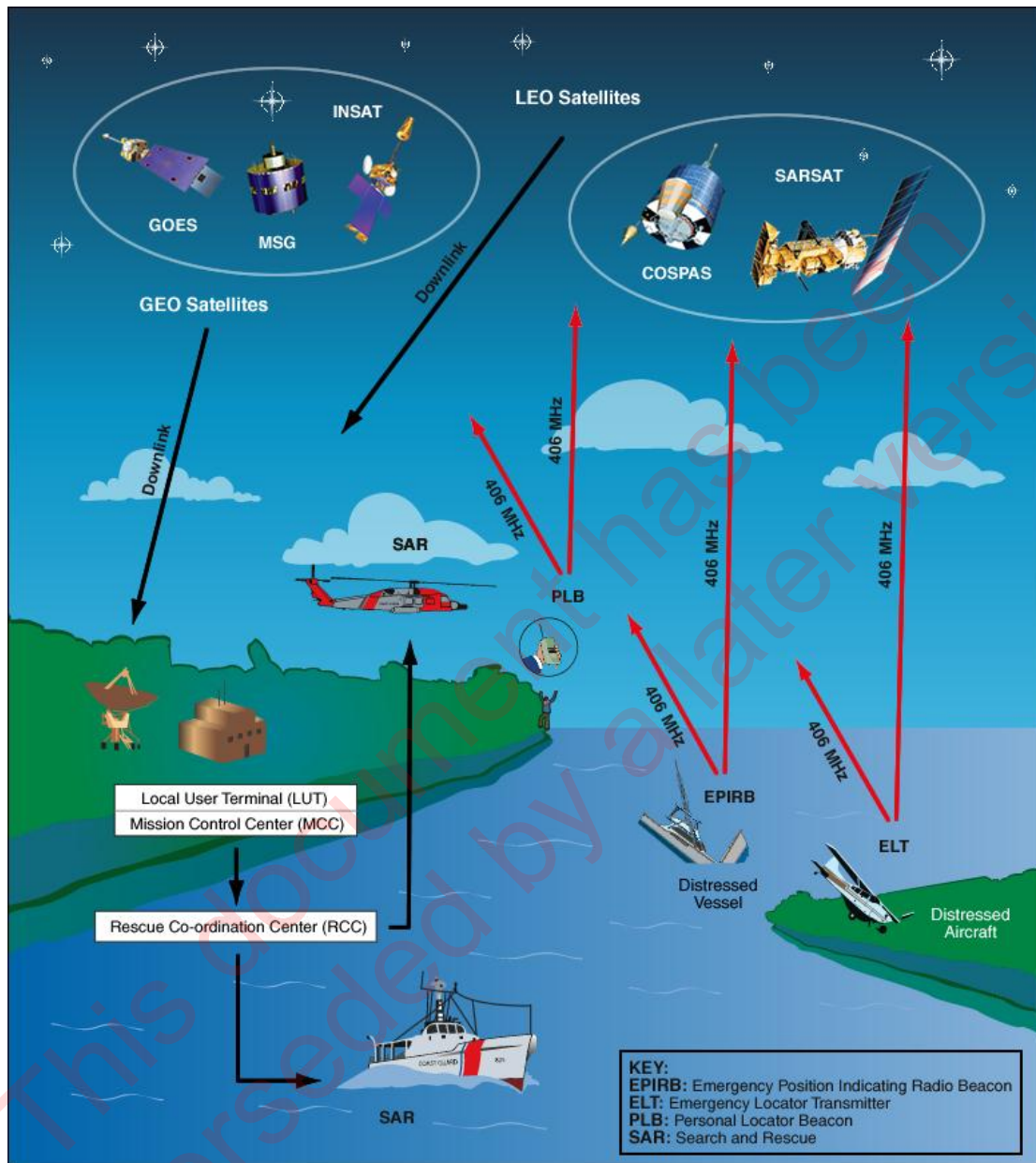
Figure 1.3: Basic Concept of the Cospas-Sarsat System
