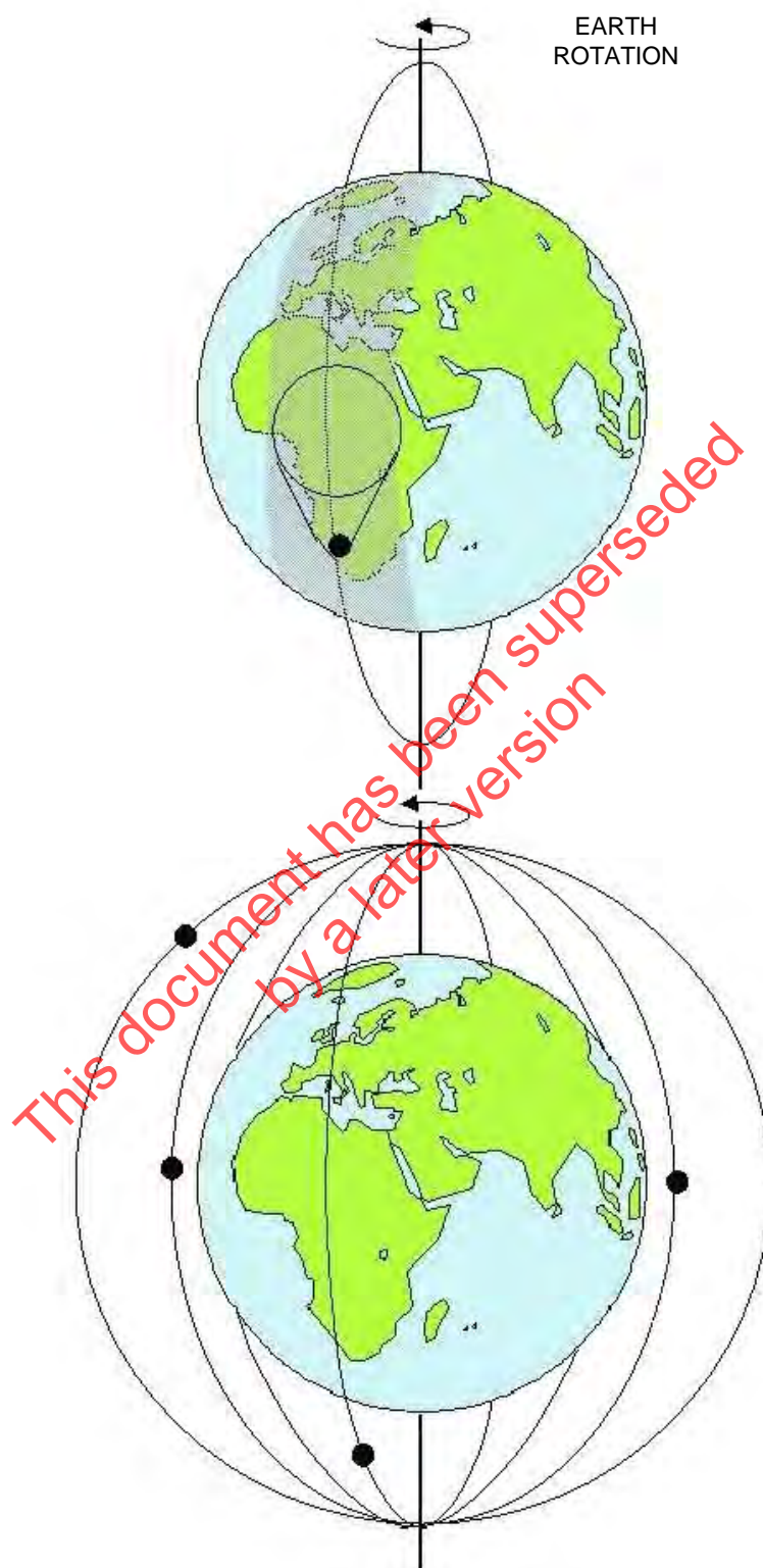
Figure 3.1: Satellites in Polar Orbit showing a single satellite (top) and a four satellite constellation (bottom)
