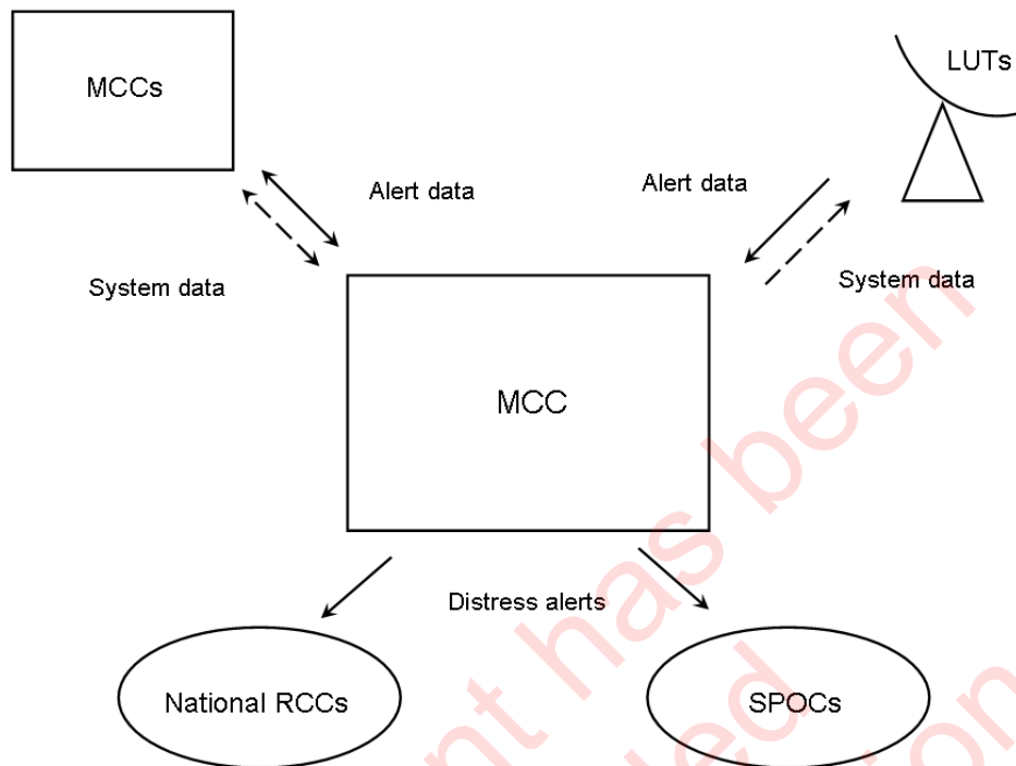
Figure 2.1: Typical Cospas-Sarsat MCC Functional Block Diagram 2
