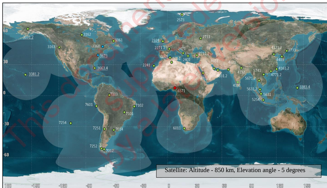
Figure B.1: Coverage Area of LEOLUTs Performing 406-MHz Routine Interference Monitoring
