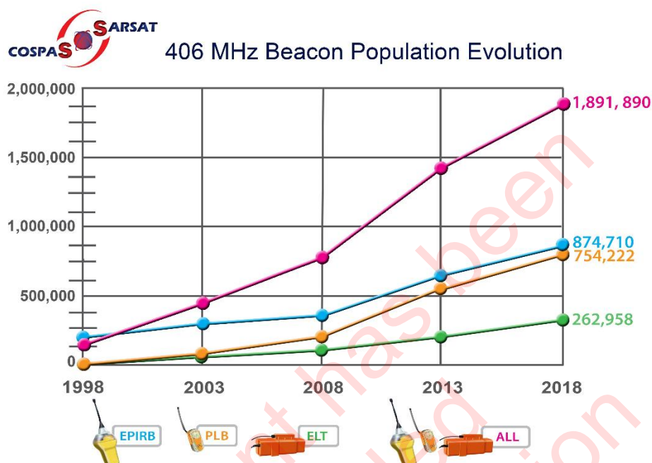
Figure 6-2: Cospas-Sarsat 406 MHz Distress Beacons
